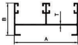
2 TRACK TOP
