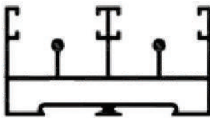
2 TRACK BOTTOM CUM PARTITION
