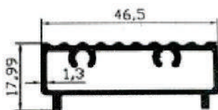
THRESHOLD
