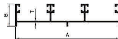
3 TRACK TOP
