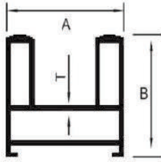
2 TRACK
