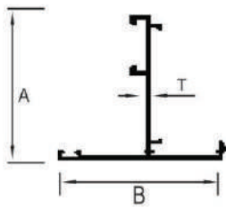
INVERSION CLIP
