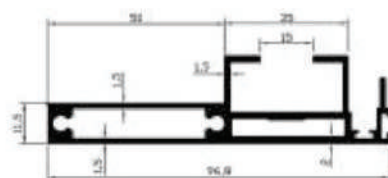
KPA INTERLOCK SINGLE GLASS
