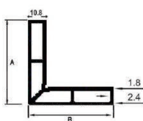
MULTI WALL ANGLE
