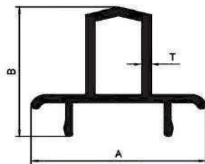
MATTING
