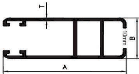
SHUTTER
