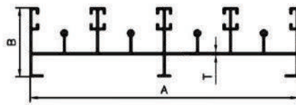
4 TRACK BOTTOM
