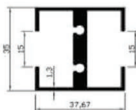
CENTER SINGLE GLASS
