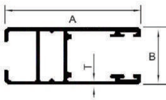
GLASS SHUTTER
