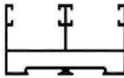
2 TRACK TOP CUM PARTITION
