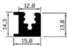
WIRE MESH ADAPTOR
