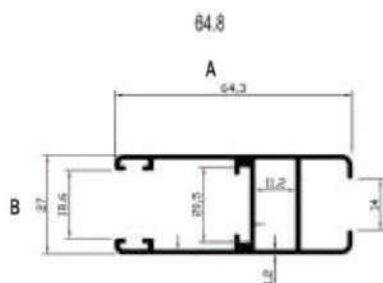
SINGLE GLASS SHUTTER
