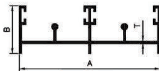
2 TRACK BOTTOM
