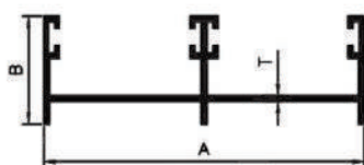
2 TRACK TOP
