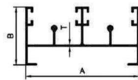
2 TRACK BOTTOM
