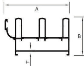
3 TRACK WITH LEG
